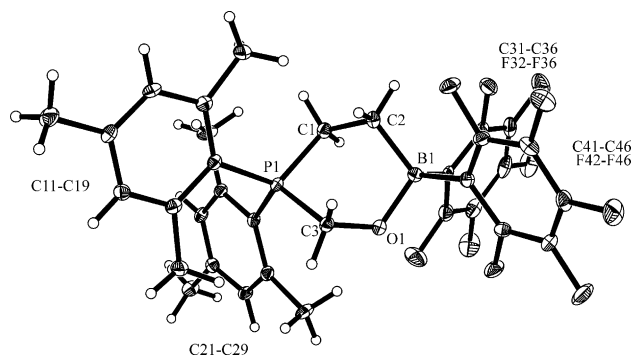
Figure 2. X-ray crystal structure analysis of the compound 5a (thermal ellipsoids are shown at 50%). Selected bond lengths (Å) and angles ( ^\circ ): C3–P1 1.847(2), C3–O1 1.400(2), O1–B1 1.503(2), P1–C3–O1 109.0(1), C3–O1–B1 117.2(1). [35]
